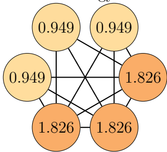
Graph 75, order 6. Total energy: 8.325
