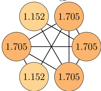
Graph 91, order 6. Total energy: 9.123
