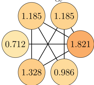
Graph 60, order 6. Total energy: 7.217
