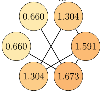
Graph 18, order 6. Total energy: 7.192
