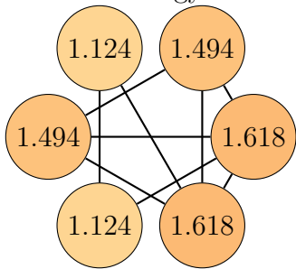
Graph 81, order 6. Total energy: 8.472
