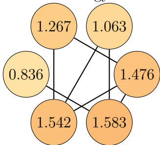
Graph 46, order 6. Total energy: 7.766
