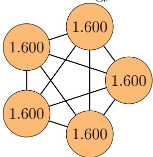
Graph 21, order 5. Total energy: 8.000
