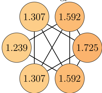
Graph 100, order 6.
