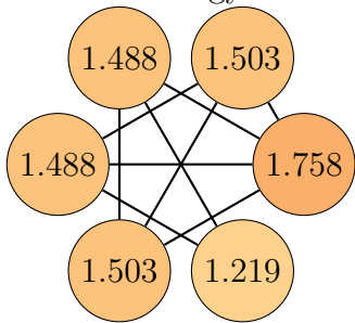
Graph 97, order 6. Total energy: 8.958
