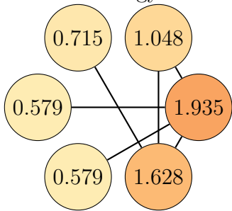
Graph 6, order 6. Total energy: 6.485
