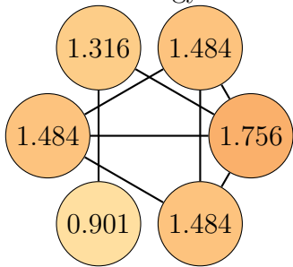
Graph 78, order 6. Total energy: 8.427
