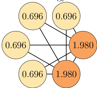
Graph 14, order 6. Total energy: 6.745
