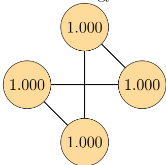
Graph 4, order 4. Total energy: 4.000
