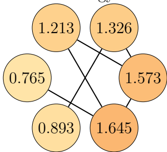
Graph 20, order 6. Total energy: 7.416
