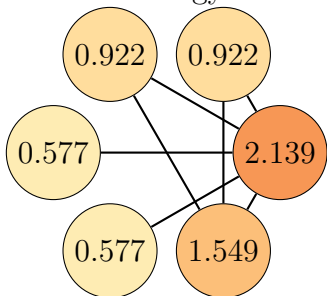
Graph 8, order 6. Total energy: 6.686
