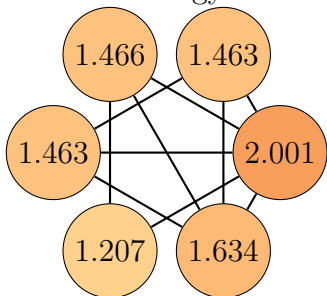
Graph 86, order 6. Total energy: 9.234
