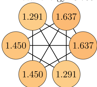
Graph 101, order 6.
