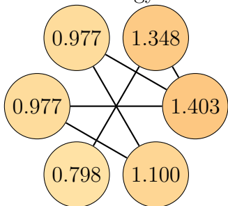
Graph 23, order 6. Total energy: 6.603
