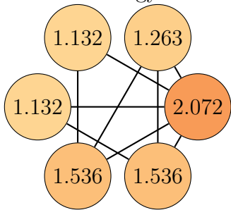
Graph 55, order 6. Total energy: 8.670
