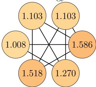
Graph 68, order 6. Total energy: 7.588
