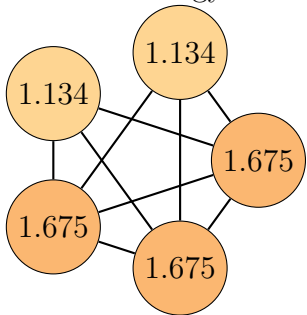
Graph 20, order 5. Total energy: 7.292
