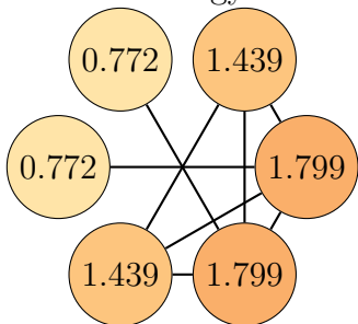
Graph 35, order 6. Total energy: 8.019
