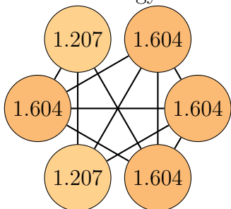
Graph 105, order 6.
