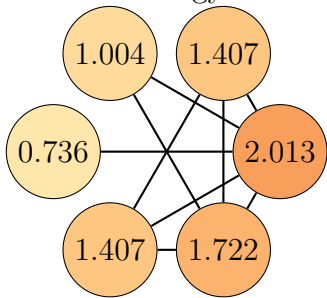
Graph 37, order 6. Total energy: 8.289
