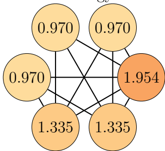
Graph 74, order 6. Total energy: 7.533
