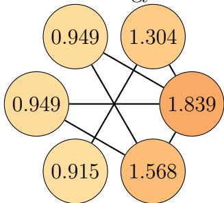
Graph 24, order 6. Total energy: 7.523
