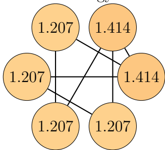
Graph 53, order 6. Total energy: 7.657
