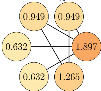
Graph 7, order 6. Total energy: 6.325
