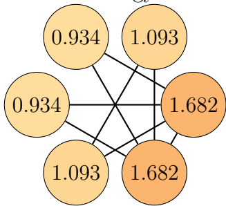
Graph 39, order 6. Total energy: 7.419
