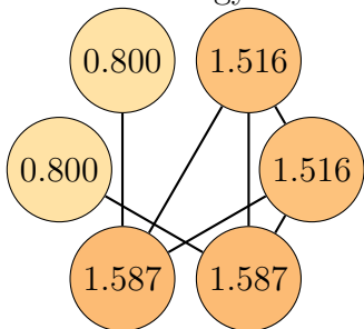
Graph 50, order 6. Total energy: 7.806
