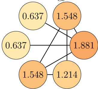
Graph 27, order 6. Total energy: 7.464
