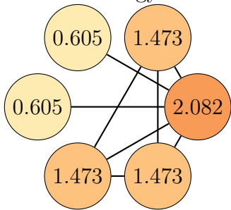
Graph 28, order 6. Total energy: 7.712
