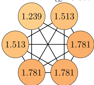
Graph 104, order 6.
