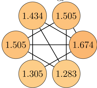
Graph 85, order 6. Total energy: 8.704
