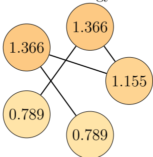
Graph 9, order 5. Total energy: 5.464
