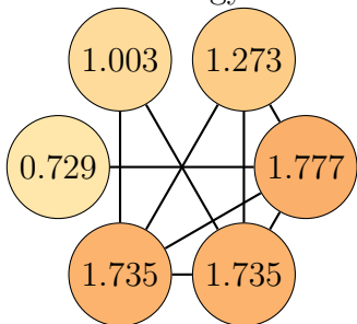
Graph 62, order 6. Total energy: 8.253
