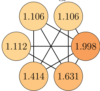
Graph 69, order 6. Total energy: 8.367
