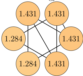
Graph 82, order 6. Total energy: 8.293
