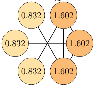
Graph 30, order 6. Total energy: 7.301
