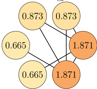
Graph 10, order 6. Total energy: 6.819
