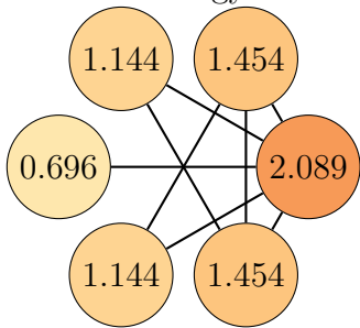
Graph 34, order 6. Total energy: 7.981
