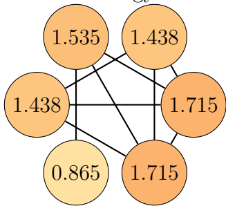
Graph 84, order 6. Total energy: 8.708
