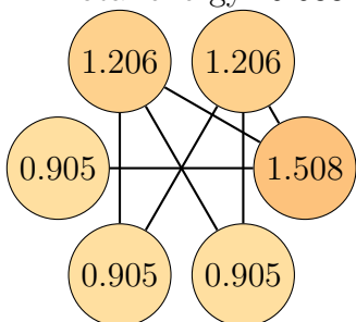
Graph 59, order 6. Total energy: 6.633
