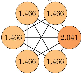
Graph 98, order 6. Total energy: 9.371
