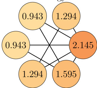
Graph 26, order 6. Total energy: 8.213
