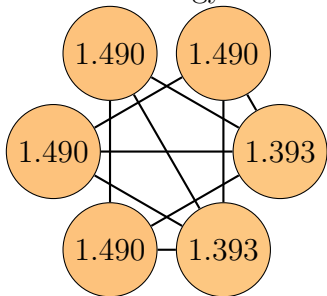
Graph 87, order 6. Total energy: 8.745
