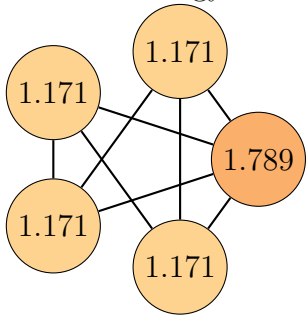
Graph 19, order 5. Total energy: 6.472
