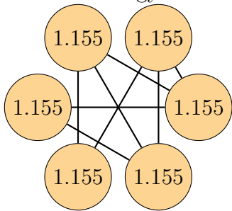
Graph 66, order 6. Total energy: 6.928
