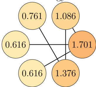
Graph 5, order 6. Total energy: 6.155
