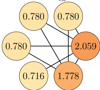
Graph 12, order 6. Total energy: 6.893
