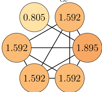
Graph 90, order 6. Total energy: 9.068
