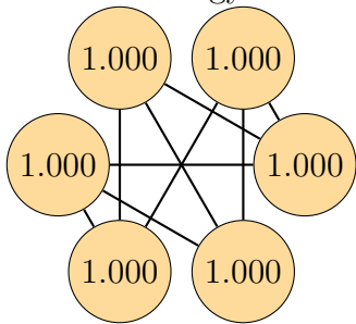
Graph 72, order 6. Total energy: 6.000
