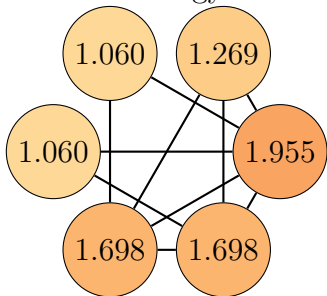
Graph 58, order 6. Total energy: 8.739
