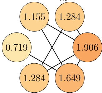
Graph 22, order 6. Total energy: 7.996
