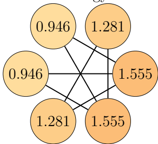
Graph 38, order 6. Total energy: 7.565
