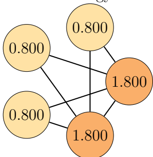
Graph 8, order 5. Total energy: 6.000
