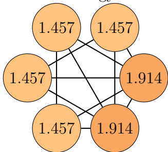
Graph 88, order 6. Total energy: 9.657
