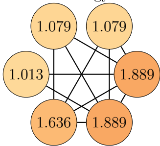
Graph 70, order 6. Total energy: 8.585
