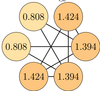
Graph 44, order 6. Total energy: 7.252
