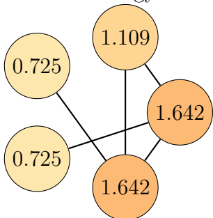
Graph 4, order 5. Total energy: 5.842
