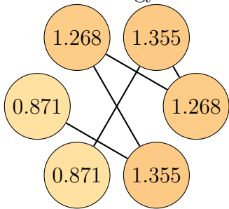
Graph 19, order 6. Total energy: 6.988
