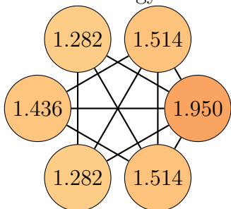
Graph 102, order 6.
