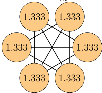
Graph 99, order 6. Total energy: 8.000
