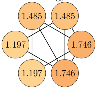
Graph 83, order 6. Total energy: 8.858
