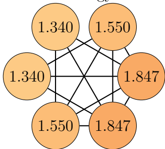
Graph 103, order 6.
