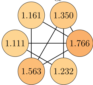
Graph 54, order 6. Total energy: 8.183
