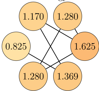
Graph 21, order 6. Total energy: 7.549
