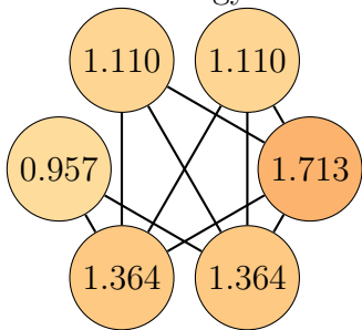
Graph 71, order 6. Total energy: 7.620
