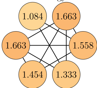
Graph 92, order 6. Total energy: 8.757
