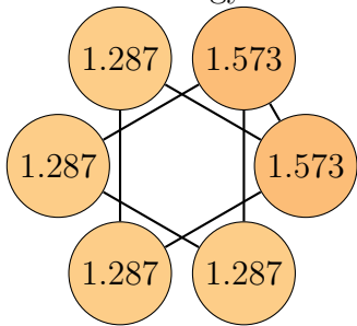
Graph 76, order 6. Total energy: 8.293
