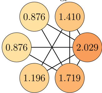
Graph 43, order 6. Total energy: 8.107
