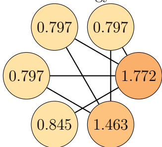
Graph 11, order 6. Total energy: 6.470
