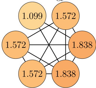
Graph 94, order 6. Total energy: 9.493
