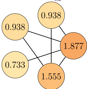
Graph 6, order 5. Total energy: 6.041
