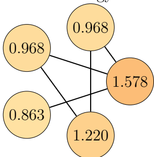
Graph 5, order 5. Total energy: 5.596
