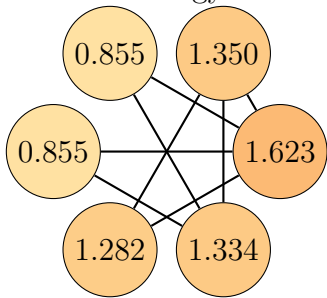
Graph 42, order 6. Total energy: 7.299
