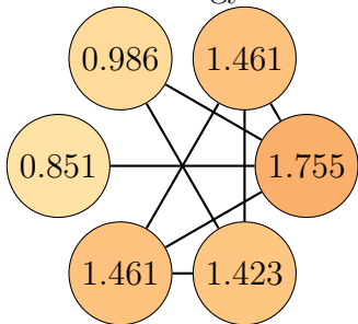
Graph 36, order 6. Total energy: 7.937
