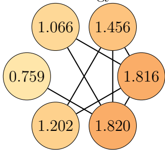
Graph 40, order 6. Total energy: 8.118
