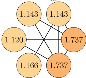
Graph 67, order 6. Total energy: 8.047
