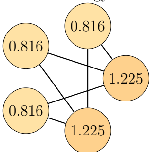
Graph 7, order 5. Total energy: 4.899
