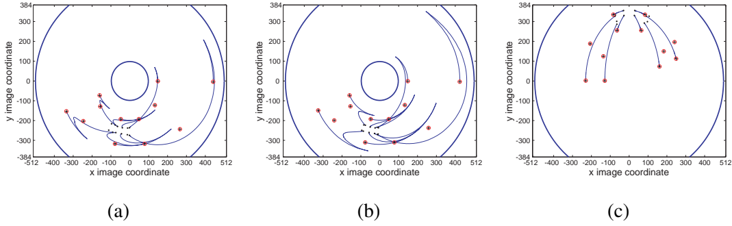
Fig. 7. Motion of the points in the image plane for three different kind of omnidirectional virtual images. (a) Hypercatadioptric. (b) Paracatadioptric. (c) Fisheye. The images depict the point features from the initial, current and target views.
