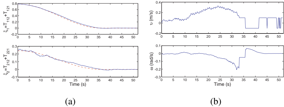
Fig. 14. Behavior of the control law using tracking of point features. (a) Outputs and their references. (b) Computed velocities.
