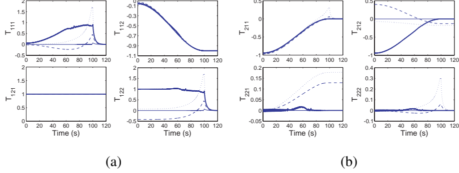
Fig. 6. Tensor elements evolution for the four cases of Fig. 4. (a) Behavior of the elements of \mathbf{T}_1 . (b) Behavior of the elements of \mathbf{T}_2 .
