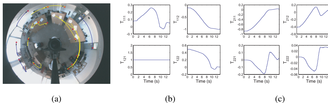
Fig. 16. Behavior of the visual measurements for the real experiments. (a) Motion of the image points. (b) Evolution of \mathbf{T}_1 . (c) Evolution of \mathbf{T}_2 .
