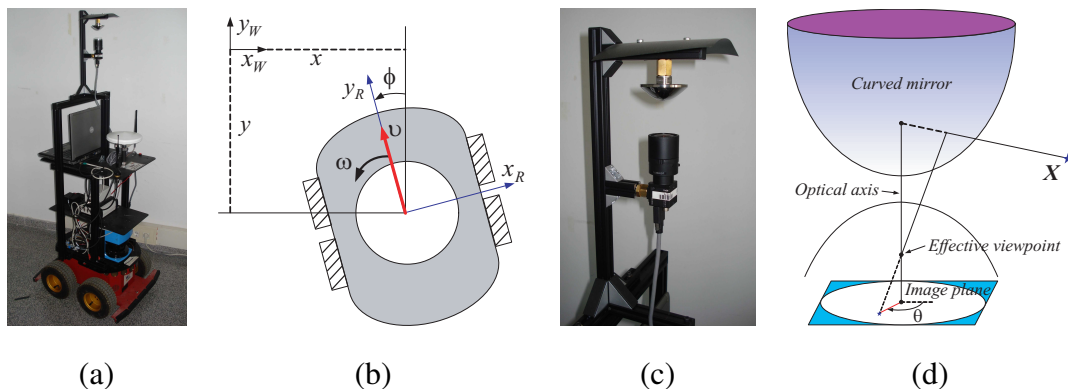
Fig. 1. Description of the robot-camera configuration. (a) Our robotic platform with the omnidirectional camera on top. (b) Robot frame definition. (c) Omnidirectional vision system with a Sony camera and Neovision mirror. (d) A generic central catadioptric system.
