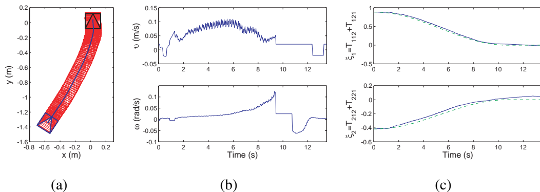
Fig. 15. Experimental results with the control law in closed loop. (a) Resultant path. (b) Computed velocities. (c) Controlled outputs. The data to plot the path is given by the robot odometry.
