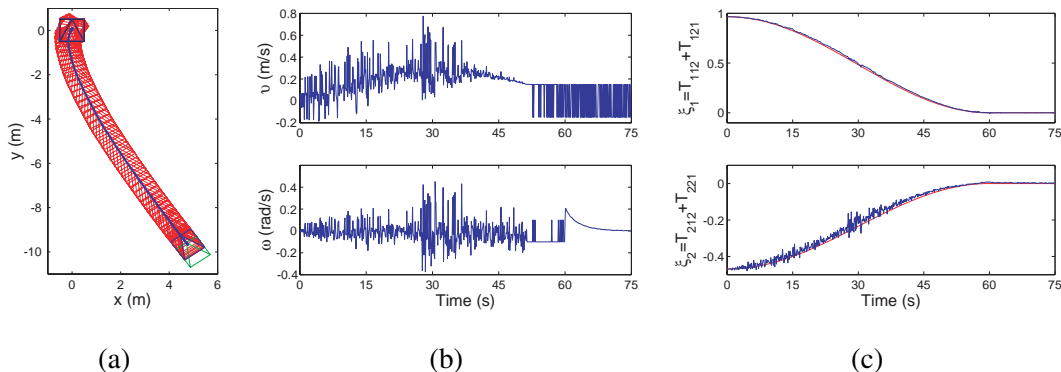
Fig. 8. Control law performance with image noise. (a) Resultant robot path. (b) Control inputs. (c) Controlled outputs.
