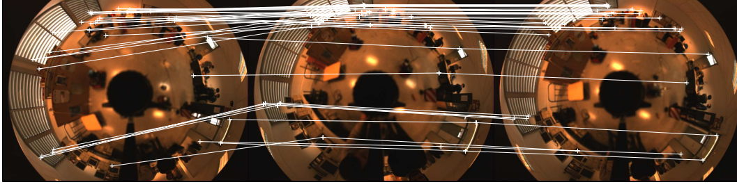
Fig. 3. Robust SIFT matching between three omnidirectional images with translation and rotation between them. The lines between images show 34 corresponding features, which have been extracted using SIFT and matched robustly to be the entries for the 1D TT estimation algorithm.
