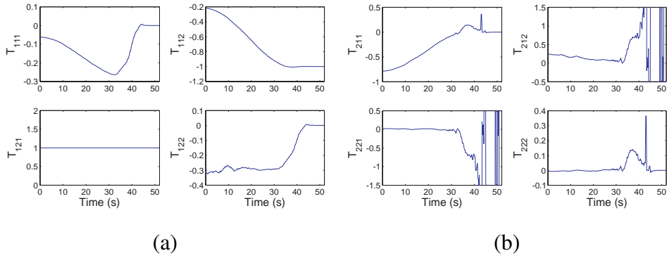
Fig. 13. Performance of the 1D TT estimation using tracking of point features. (a) Behavior of the elements of \mathbf{T}_1 . (b) Behavior of the elements of \mathbf{T}_2 .
