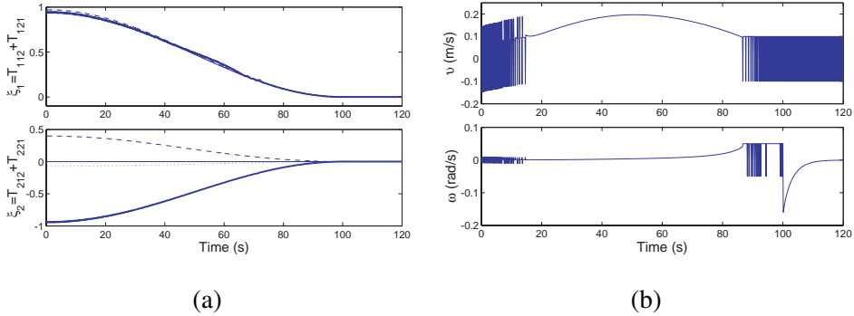
Fig. 5. Control law performance. (a) Controlled outputs for the four cases of Fig. 4. (b) Example of the computed velocities for initial location (-5, -12, -30^\circ) .
