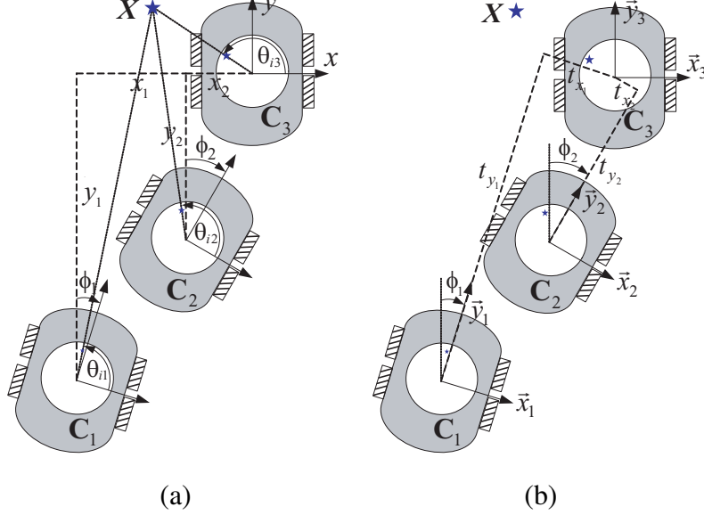
Fig. 2. Framework of the three-view geometry. (a) Global reference definition with origin in the third view and bearing measurements \theta of a feature. (b) Relative location between cameras with a fixed reference frame on each view.
