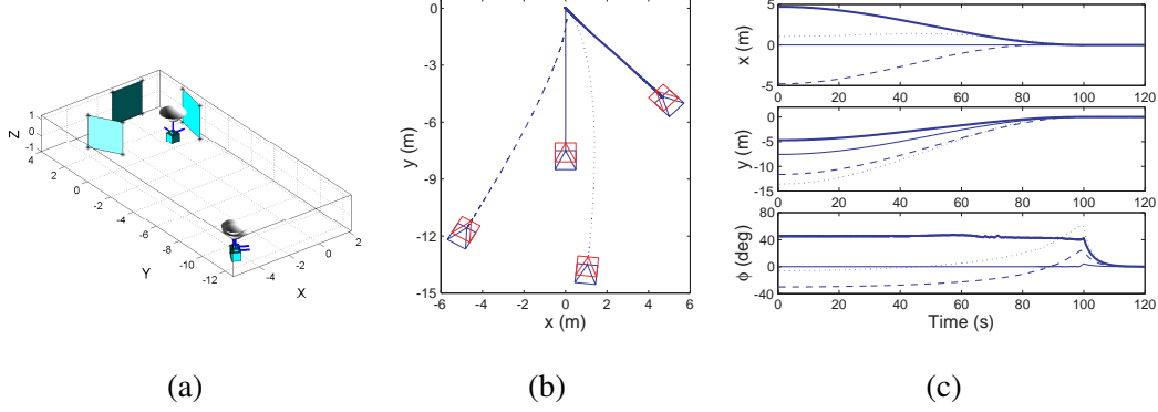
Fig. 4. Simulation results with synthetic images. (a) 3D scene. (b) Paths on the plane. (c) State variables of the robot.
