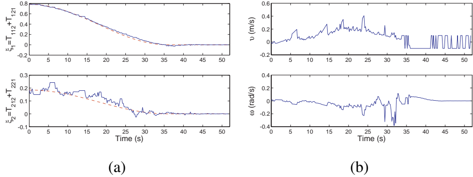
Fig. 11. Behavior of the control law using SIFT features. (a) Outputs and their references. (b) Computed velocities.
