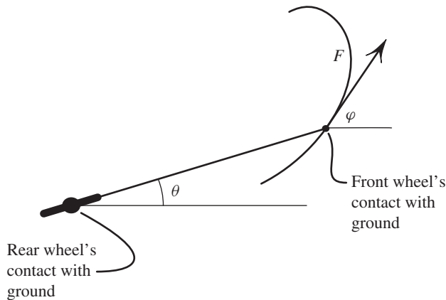
Figure 15. Notations to proof of Lemma 4.1
