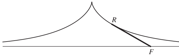
Figure 1. The classical tractrix
