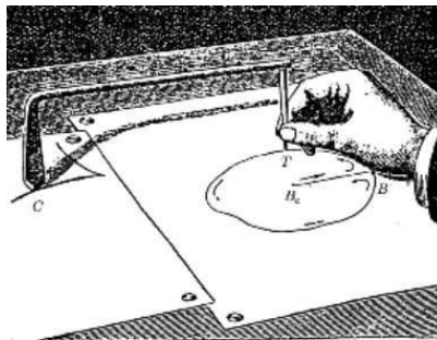
Figure 2. The Prytz Planimeter
